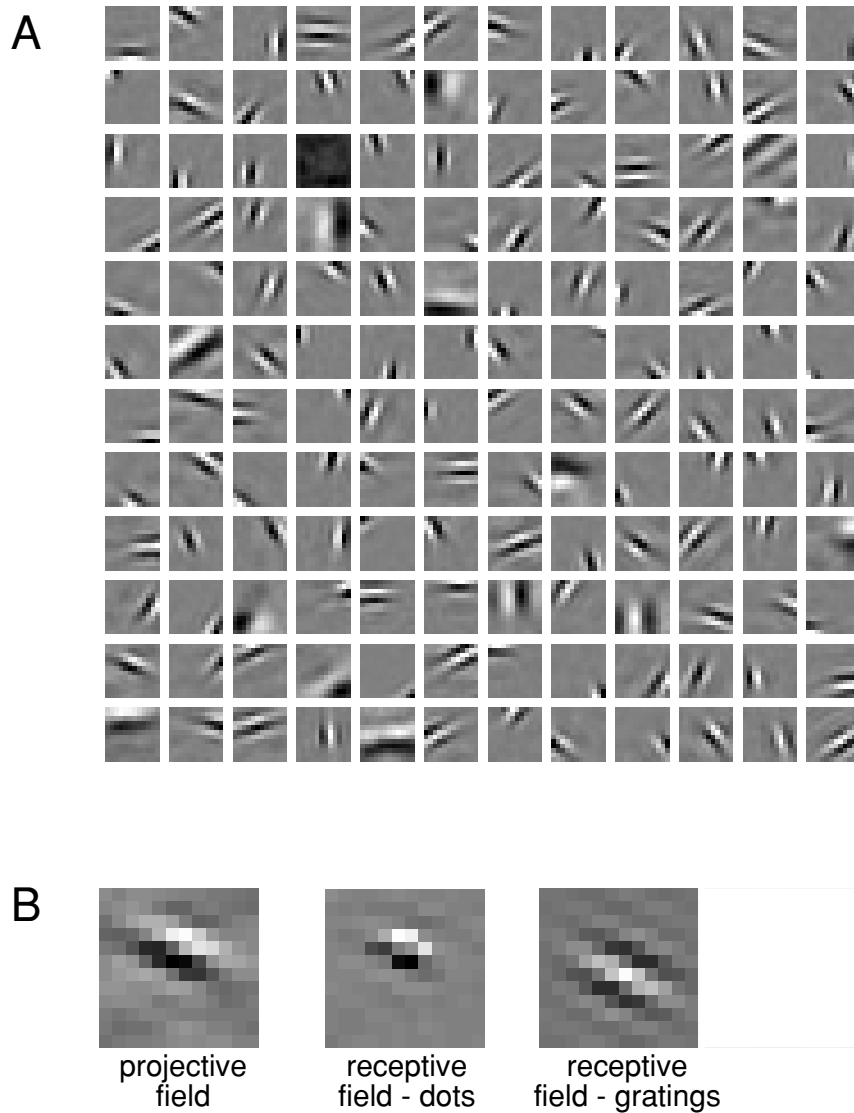
Figure 10.7 Projective and receptive fields for a sparse coding network with N_u = N_v = 144 . (A) Projective fields \mathbf{G}_{ab} with a indexing representational units (the components of \mathbf{v} ), and b indexing input units \mathbf{u} on a 12 \times 12 pixel grid. Each box represents a different a value, and the b values are represented within the box by the corresponding input location. Weights are represented by the gray-scale level, with gray indicating 0. (B) The relationship between projective and receptive fields. The left panel shows the projective field of one of the units in A. The middle and right panels show its receptive field mapped using inputs generated by dots and by gratings, respectively. (Adapted from Olshausen & Field, 1997.)
