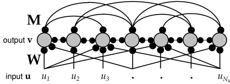
Figure 8.6 A network with multiple output units driven by feedforward synapses with weights W , and interconnected by recurrent synapses with weights M .
